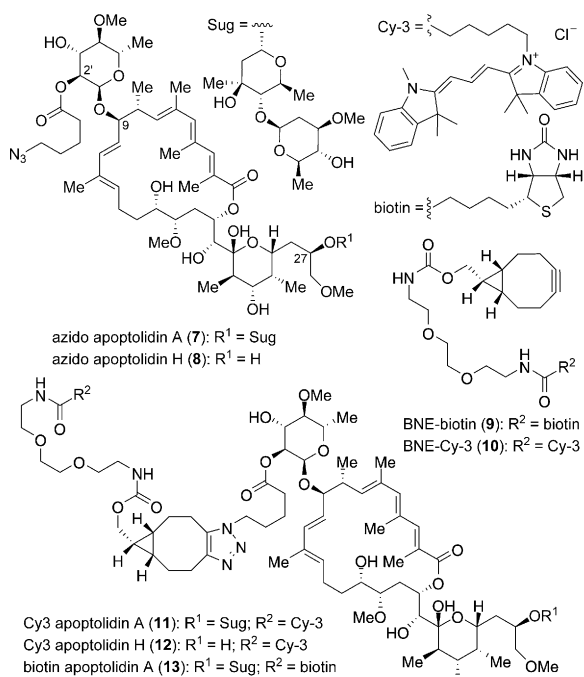
Figure 3. Azido apoptolids, strained alkyne tagging reagents, and derived probes.
