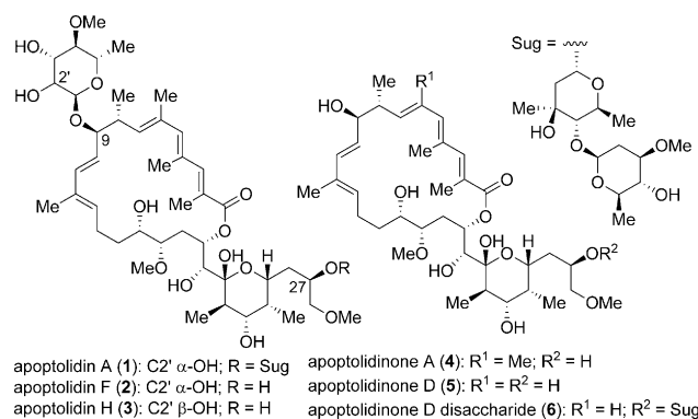
Figure 1. Members of the apoptolidin family of macrolides.
