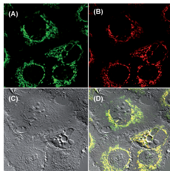
Figure 4. Co-staining Cy3 apoptolidin A and MitoTracker in H292 cells. Fluorescence images of MitoTracker (A), 11 (B), DIC image (C), and merged image (D) are shown.
