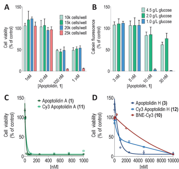
Figure 2. Analysis of apoptolidin toxicity in H292 cell line. A) Dependence of cytotoxic and cytostatic effects of 1 on cell confluency as measured by initial number of cells per well on a 96 well plate. B) Effect of cell growth media of varying glucose concentrations on 1 cytotoxicity. C) Cell viability assay for 1 and 11 . D) Cell viability assay for 3 , 12 , and 10 evaluated using optimized conditions.
